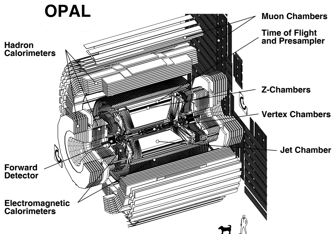
Figure 3.2: A schematic of the OPAL detector at LEP.
