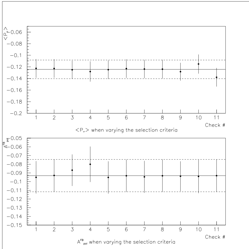
Figure 5.4: This figure shows \langle P_\tau \rangle and A_{\text{pol}}^{\text{FB}} extracted from the 1990-94 data sample when the selection criteria are varied. The solid lines show the nominal values \langle P_\tau \rangle and A_{\text{pol}}^{\text{FB}} extracted from this analysis and the dotted lines show the statistical errors of these values. The systematic checks shown in this figure are explained in table 5.3.
