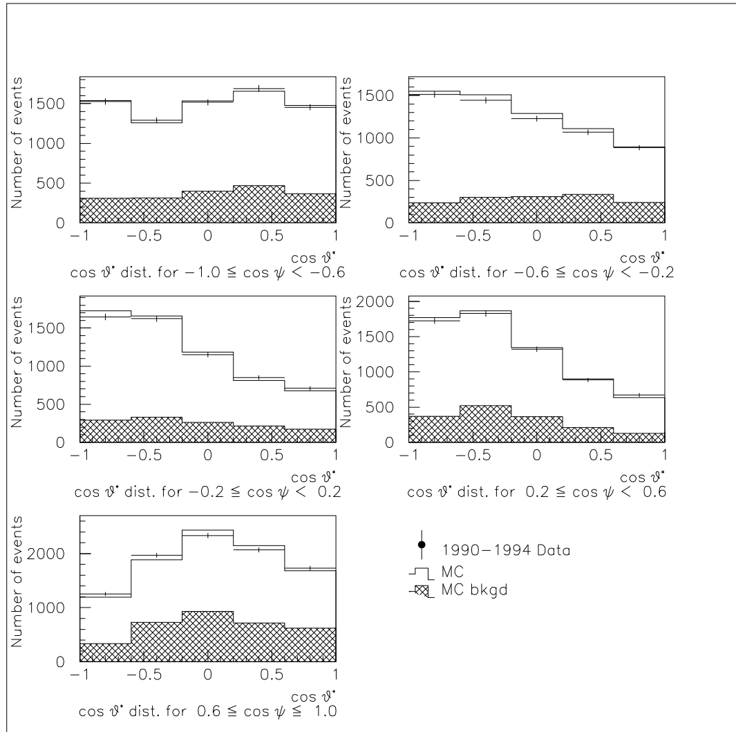
Figure 4.15: This figure shows the reconstructed quantity \cos \theta^* in five bins of reconstructed \cos \psi for both data and Monte Carlo candidates.
