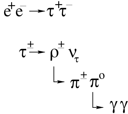
Figure 4.1: The decay chain of the \rho^{\pm}(770) to a charged pion and neutral pion with the subsequent decay of the neutral pion to two photons.
