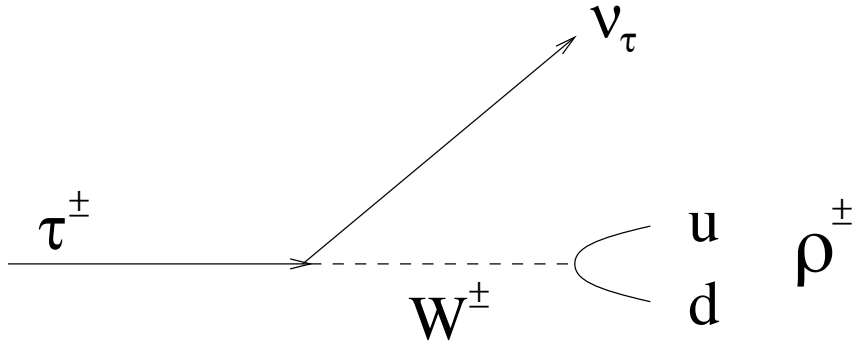
Figure 2.11: The weak decay \tau^\pm \rightarrow \rho^\pm \nu_\tau .
