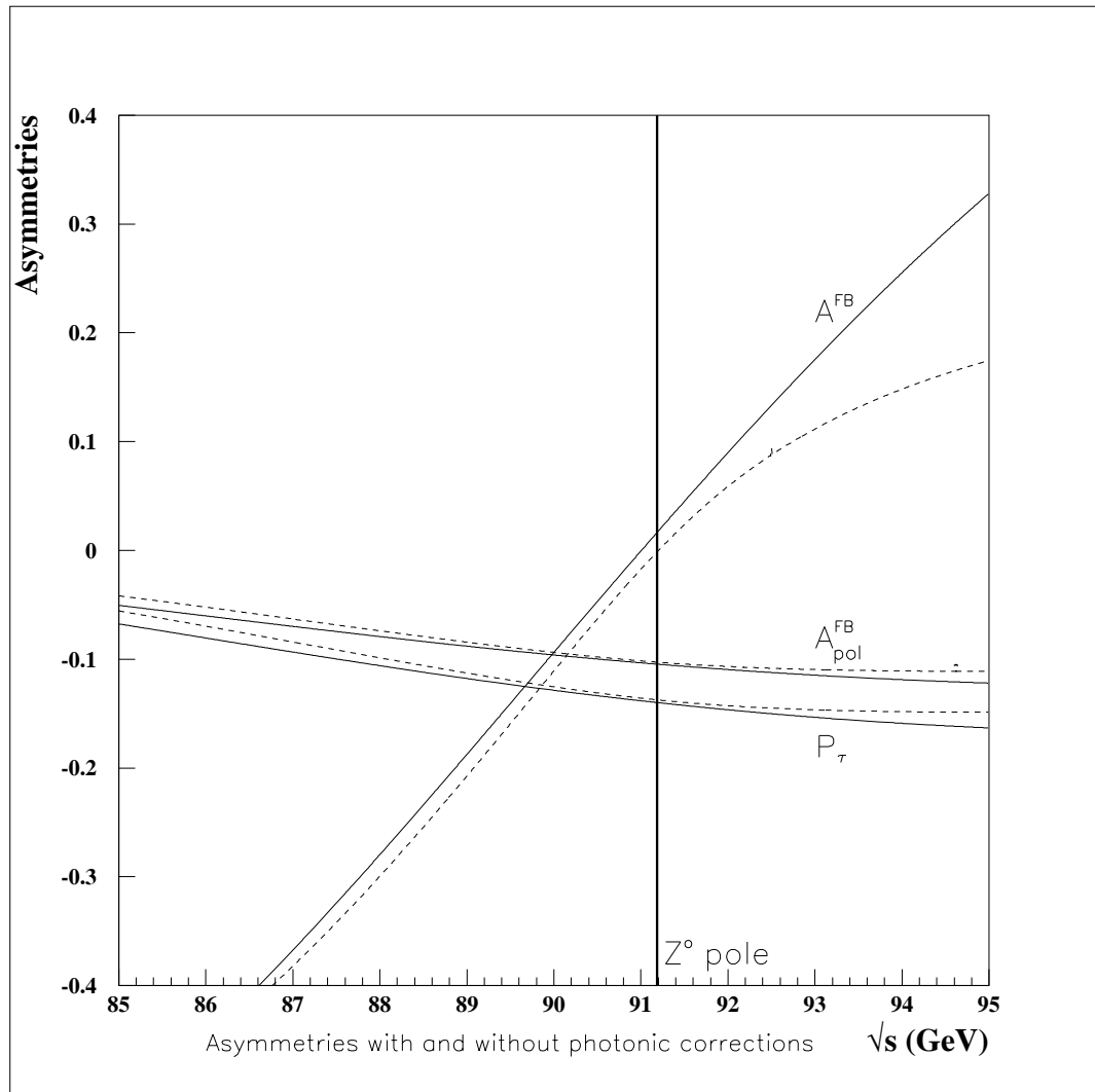
Figure 2.10: The effect of applying the photonic corrections to the calculation of the asymmetries A^{\text{FB}} , \langle P_{\tau} \rangle , and A^{\text{FB}}_{\text{pol}} are shown by using the ZFITTER program [10] to calculate radiative corrections (the dashed lines in this figure).
